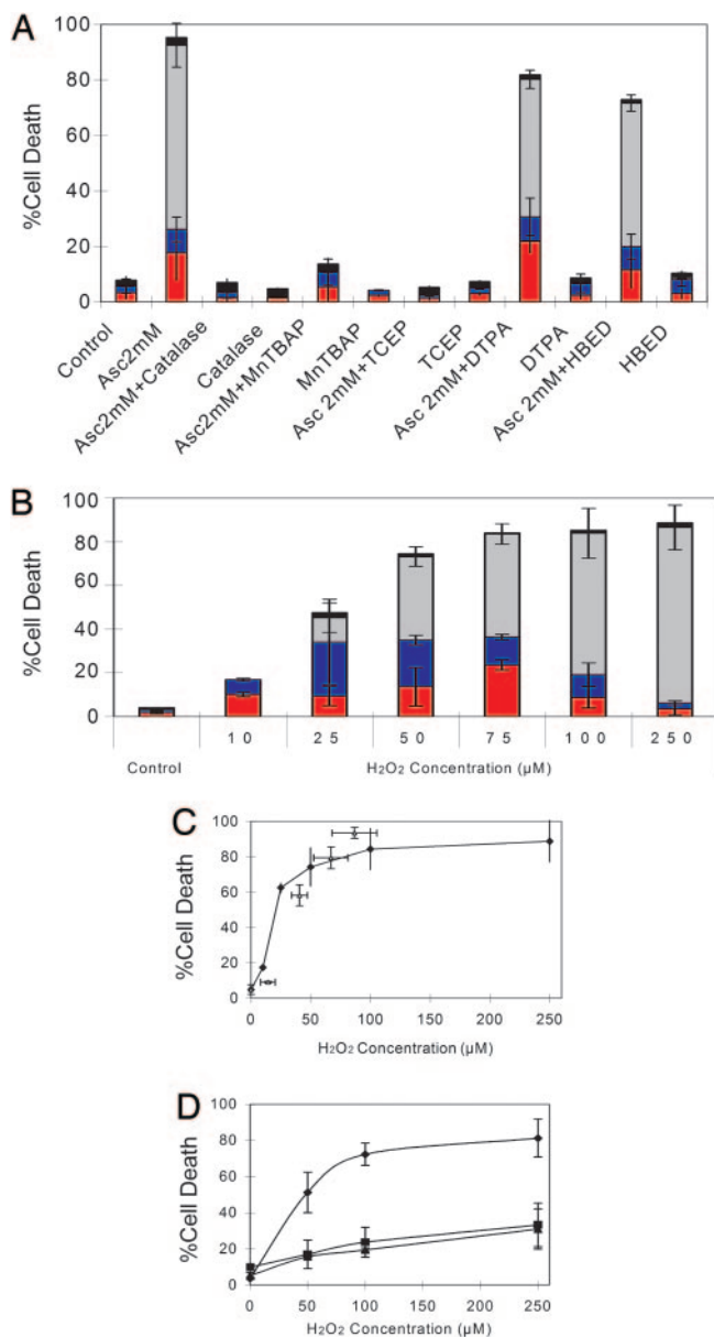
Fig. 3. Extracellular ascorbate kills human Burkitt's lymphoma cells by generating H 2 O 2 . Cell death determined and symbolized as in Fig. 2; H 2 O 2 measured by oxygen electrode (see Materials and Methods ). (A) Effects of reactive oxygen species quenchers/scavengers, reducing agent, and metal chelators on ascorbate-mediated cell death. The following (final concentrations) were preincubated with cells for 30 min before exposure to ascorbate (2 mM): catalase (100 \mu g/ml); tetrakis (4-benzoic acid) meso-substituted manganoporphyrin (MnTBAP) (100 \mu M); Tris (2-carboxyethyl) phosphine hydrochloride (TCEP) (500 \mu M); diethylenetriamine-pentaacetic acid (DTPA) (1 mM); and N,N' -bis(2-hydroxybenzyl)ethylenediamine- N,N' -diacetic acid (HBED) (50 \mu M). (B) Type and amount of cell death as function of added H 2 O 2 (final concentrations). (C) Cell death as a function of added H 2 O 2 for 1 h ( \blacklozenge ) or mean H 2 O 2 concentration generated by 0.2–2 mM ascorbate during a 1-h incubation ( \triangle ). (D) Cell death in human Burkitt's lymphoma cells ( \blacklozenge ), normal lymphocytes ( \blacksquare ), and normal monocytes ( \blacktriangle ) as function of added H 2 O 2 (final concentrations).
